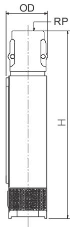
DIMENSIONS & WEIGHT
